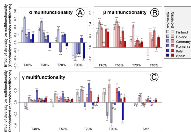
Fig. 3. Scale-dependent effects of biodiversity on forest ecosystem multifunctionality are generally consistent across countries. Bars represent the standardized regression coefficients of \alpha -diversity (blue) and \beta -diversity (red) in LMMs explaining \alpha - (A), \beta - (B), or \gamma - (C) multifunctionality. Multifunctionality was quantified at different scales using a threshold approach, with thresholds of 40%, 50%, 70%, and 90%. In addition, sum-based \gamma -multifunctionality was calculated as the sum of scaled (between 0 and 1) individual function values. Diversity measures were calculated based on individuals of target tree species.
